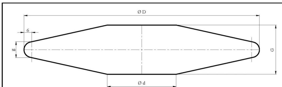
The discus specifications according to the IAAF rules
