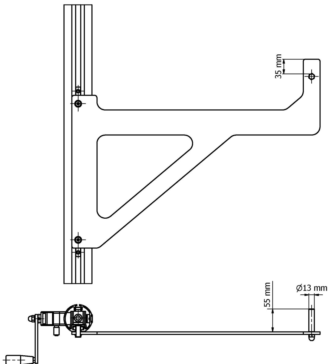
STT15-63 crossbar support view
